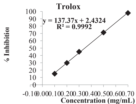
Figure 2. Calibration plot for ABTS assay
