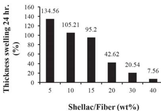
Fig. 4 The relationship between the thickness swelling in the 24th hour and the amount of binder
